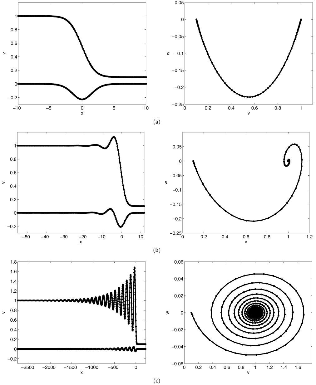
Fig. 1. Images of the profiles and their derivatives (left) and corresponding phase portraits (right) for an adiabatic monatomic gas ( \gamma = 5/3 ) with v_+ = 0.1 and d varying (note d_* \approx 0.259 ). We demonstrate (a) monotone profiles with d = 0.2 , (b) nonmonotone profiles which are mildly oscillatory with d = 2 , and (c) nonmonotone profiles that are highly oscillatory with d = 200 .
