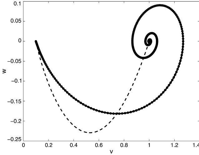
Fig. 2. Two phase portraits for an adiabatic monatomic gas ( \gamma = 5/3 ) for v_{\pm} = 0.1 . The dark line corresponds to a nonmonotone profile with d = 5 and the dotted line is the zero-capillarity profile w = \phi(v) . Note that the dotted curve intersects the dark one at its minimum. Hence to bound the derivative of the nonmonotone profile, we need only bound the derivative of the monotone profile.
